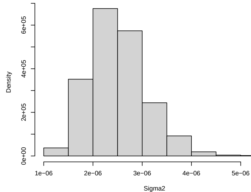
Density of Sigma2
