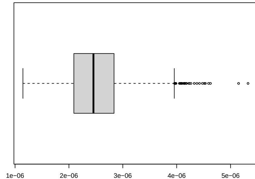
Box plot of Sigma2
